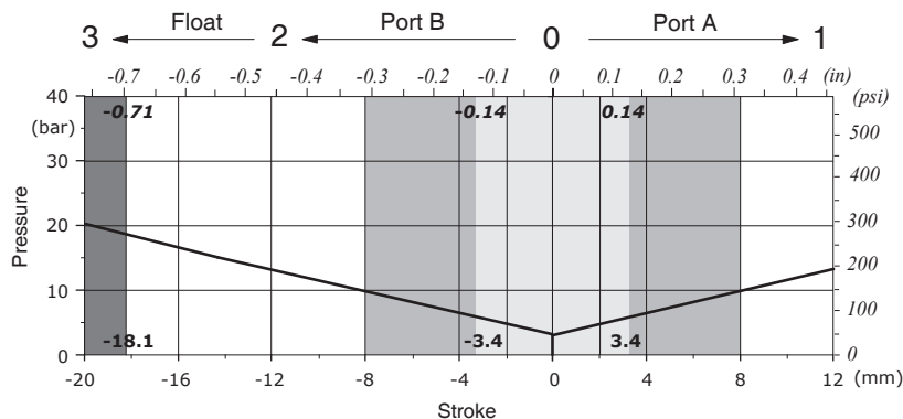
Pressure-stroke diagram
