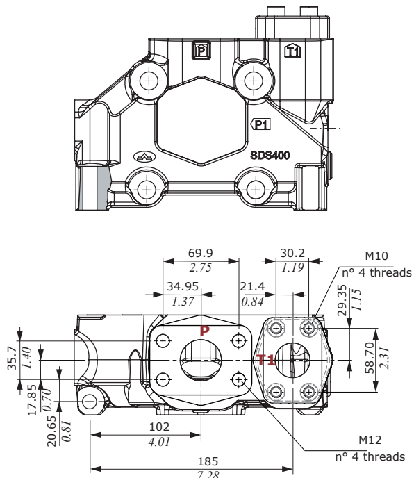
AD FS3M type (ISO flange connection)
