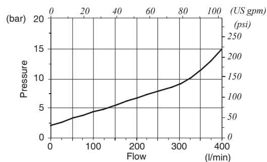
EL valve pressure drop
