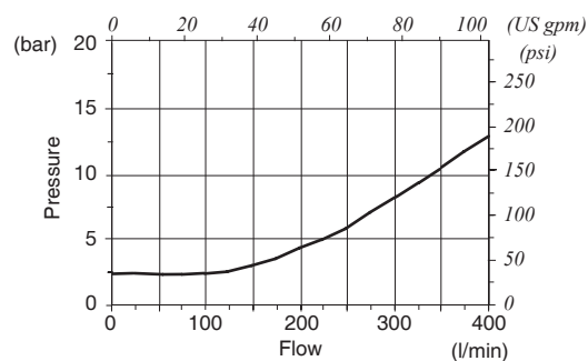
L valve pressure drop
