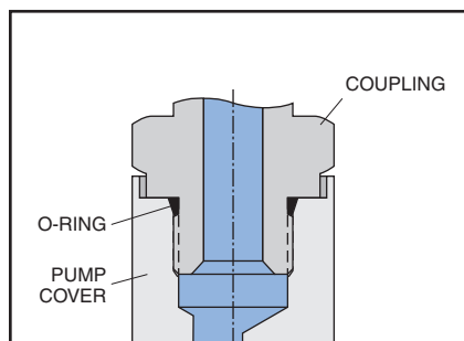
Typical S.A.E. Straight Thread port connection
